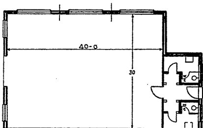
THE »NEST« FACTORY UNIT. Scale: 20 feet to 1 inch
